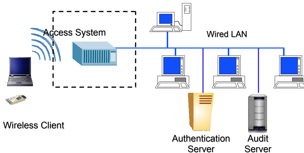
Figure 4: Example WLAN Access System with Authentication and Audit Servers
