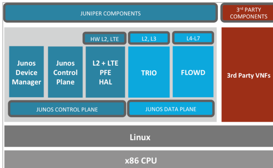
Figure 1 NFX150 Architecture
