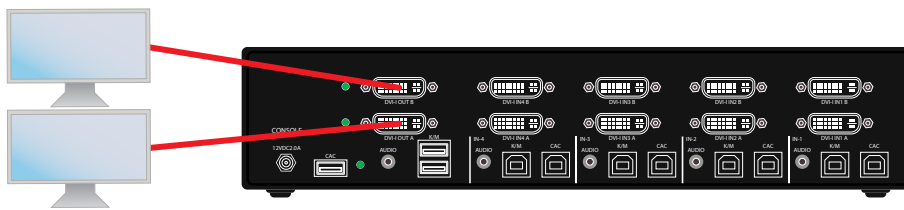
Figure 7-2: KVS4-2004DX
