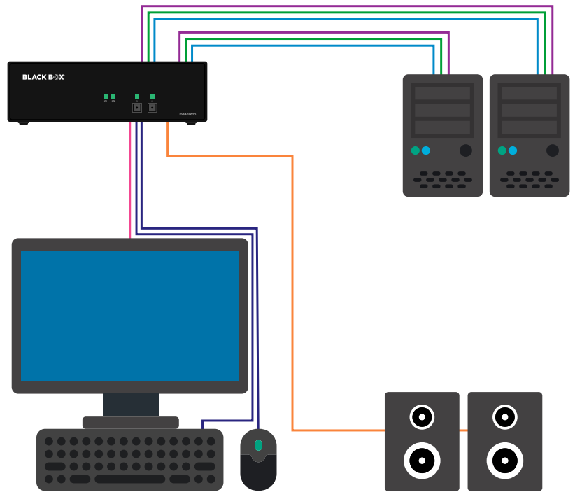
Figure 8-1: KVS4-1002D
