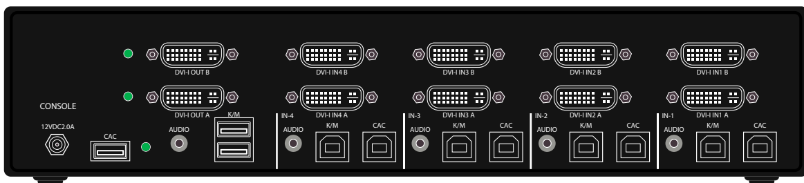
Figure 4-2: KVS4-2004DX Rear panel
