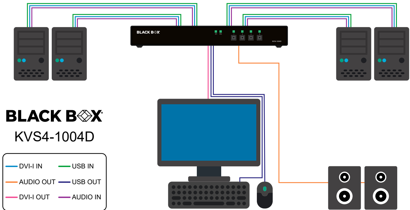
Figure 6-1: KVS4-1004D
