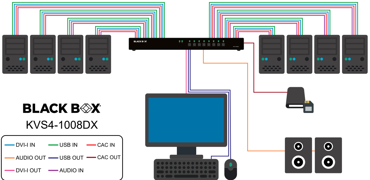
Figure 8-2: KVS4-1008DX
