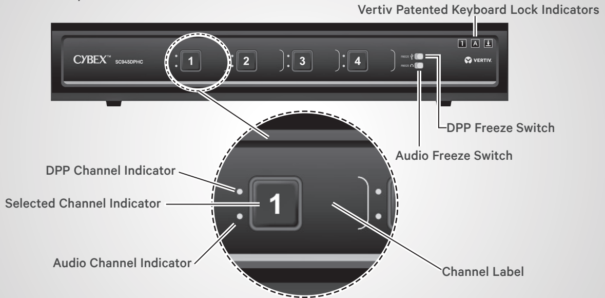
Front Panel of the Cybex™ SC945DPHC KVM Switch Shown
