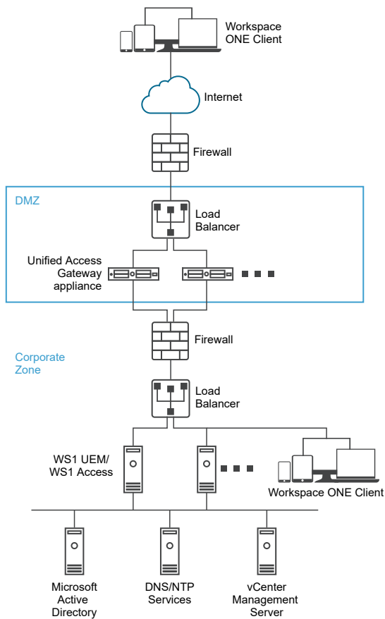
Figure 4-2. Unified Access Gateway Appliance Pointing to Workspace ONE Access
