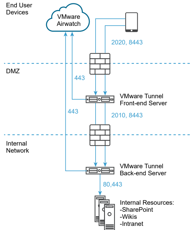
Figure 4-6. VMware Tunnel Multi-Tier Deployment: Proxy and Per-App Tunnel
