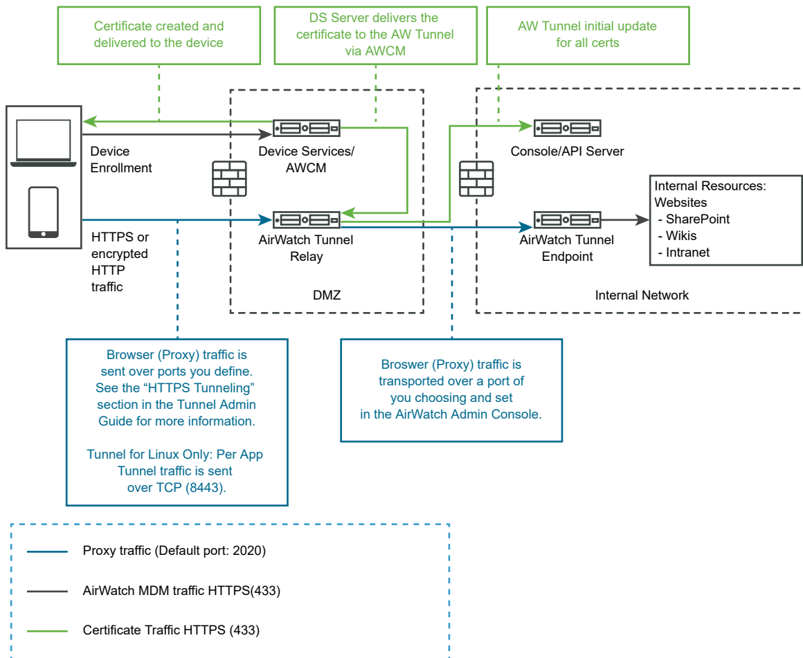
Figure 4-7. On-premises configuration for Relay-Endpoint deployments
