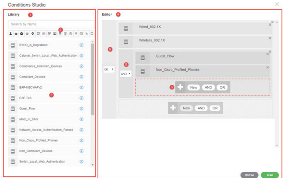
Figure 42: Conditions Studio
