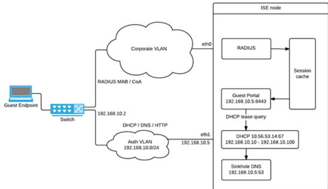
Figure 31: Auth VLAN Connected to Cisco ISE Node
