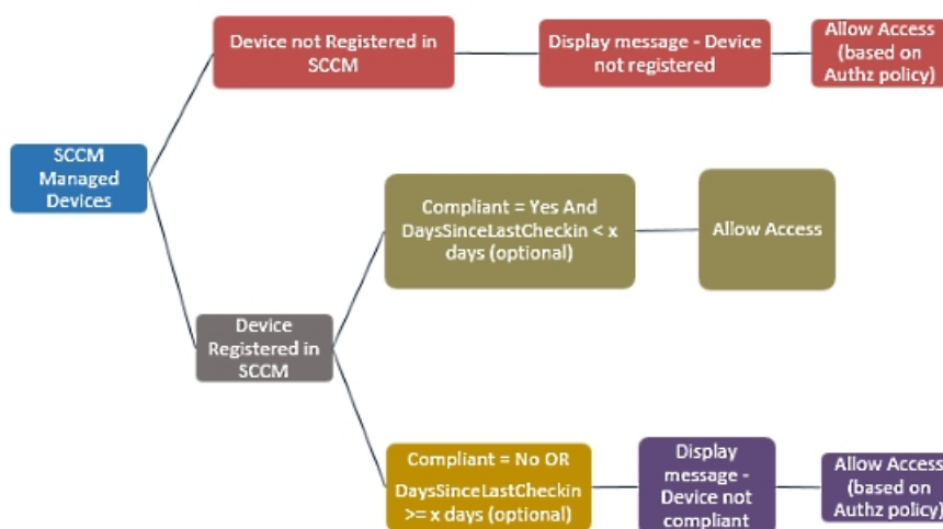
Figure 37: SCCM Workflow
