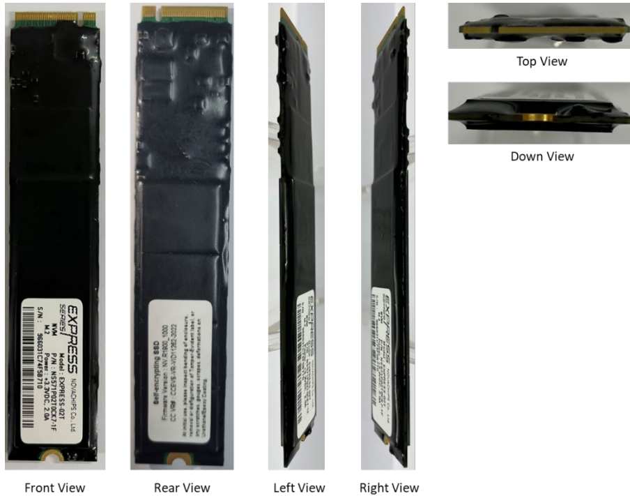
Figure 12. M.2 22110 PCIe/NVMe SSD Module (NS571P02T0CK7-1F, NS579P04T0VK7-1F)
