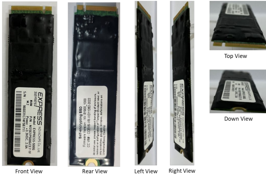
Figure 11. M.2 2280 PCIe/NVMe SSD Module (NS561P500GCE7-1F)
