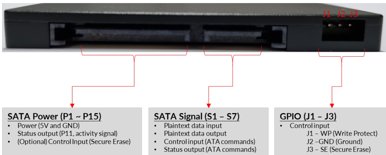
Figure 14. Ports description of 2.5" SATA products (NS361P500GCCR-1F, NS371P01T0CC1-1F, NS371P02T0CC1-1F, NS371P04T0CC1-1F, NS371P08T0CC0-1F, NS371P10T0CC0-1F, NS379P16T0VCO-1F, and NS379P20T0VCO-1F)
