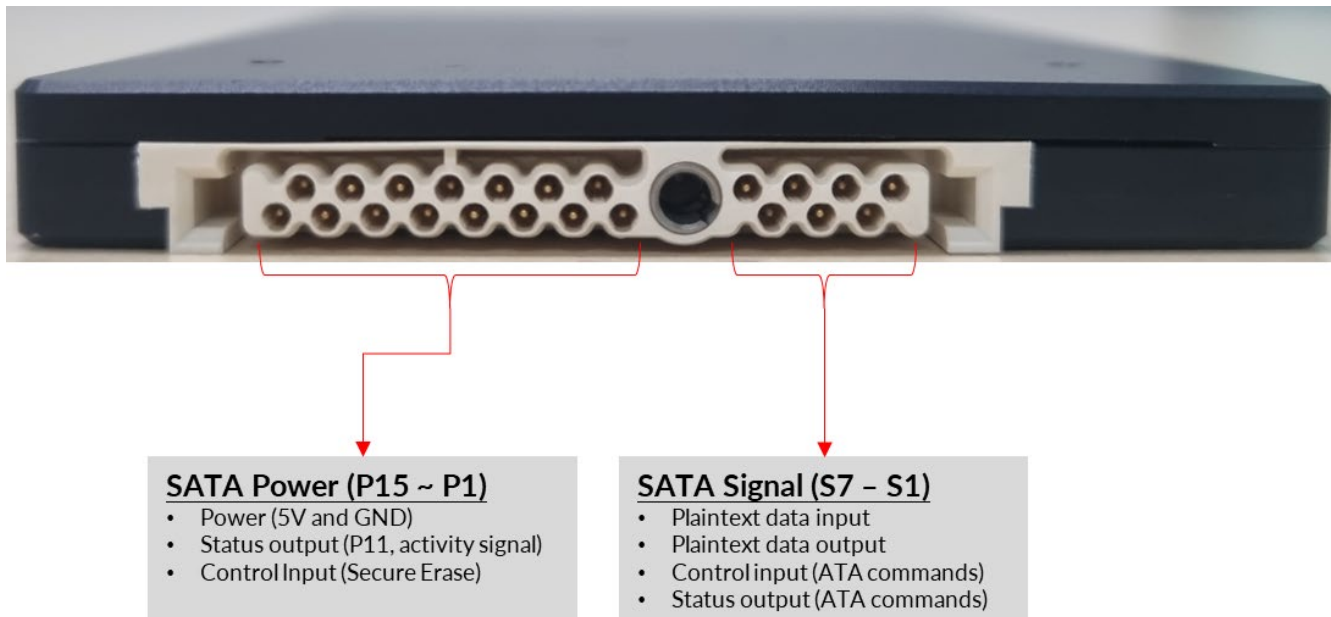
Figure 15. Ports description of 2.5" RSATA products (NS361P250GCC0-1S, NS361P500GCC0-1S, NS369P01T0VC0-1S, NS369P02T0VC0-1S)
