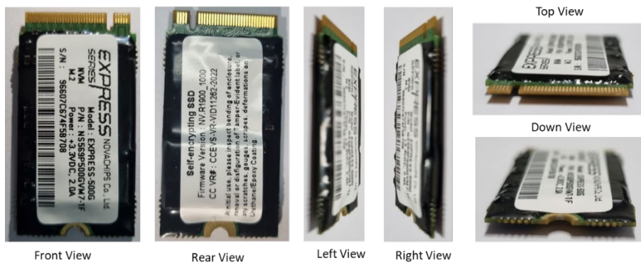
Figure 10. M.2 PCIe/NVMe 2242 SSD Module (NS569P500GVM7-1F)
