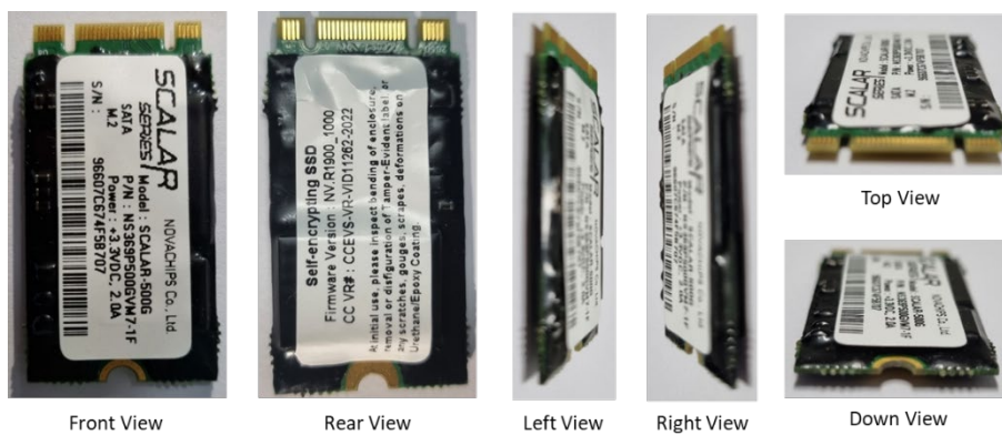
Figure 6. M.2 SATA 2242 SSD Module (NS361P125GCM7-1F, NS369P250GVM7-1F, NS369P500GVM7-1F)
