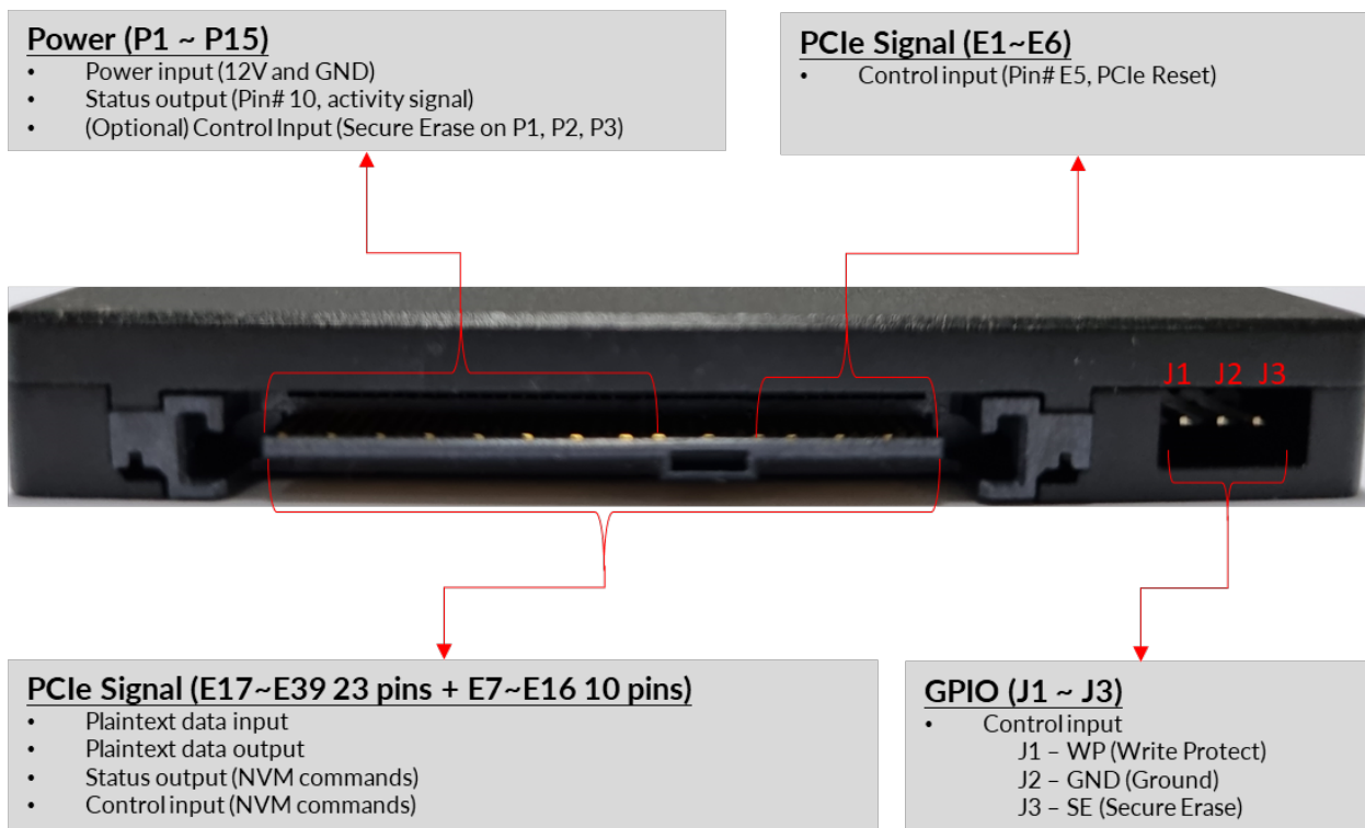
Figure 20. Ports description of PCIe U.2 SSD module (NS571P01TOCC0-1F, NS571P02TOCC0-1F, NS571P04TOCC0-1F, NS571P08TOCC0-1F)
