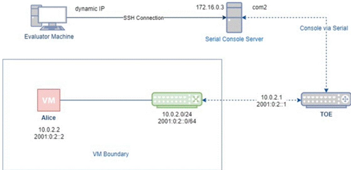
Figure 2 - Test Environment
