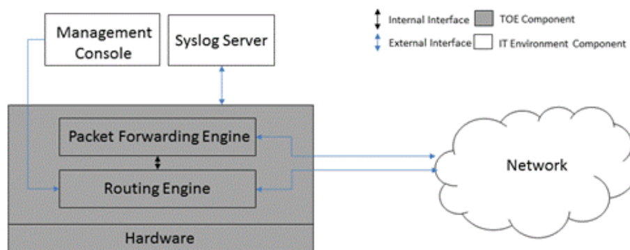
Figure 1 - ACX5448-M TOE Boundary
