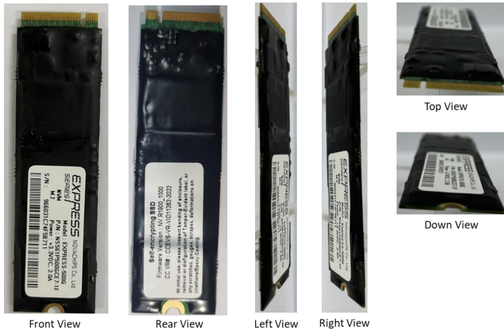
Figure 13. M.2 2280 PCIe/NVMe SSD Module (NS561P500GCE7-1F)
