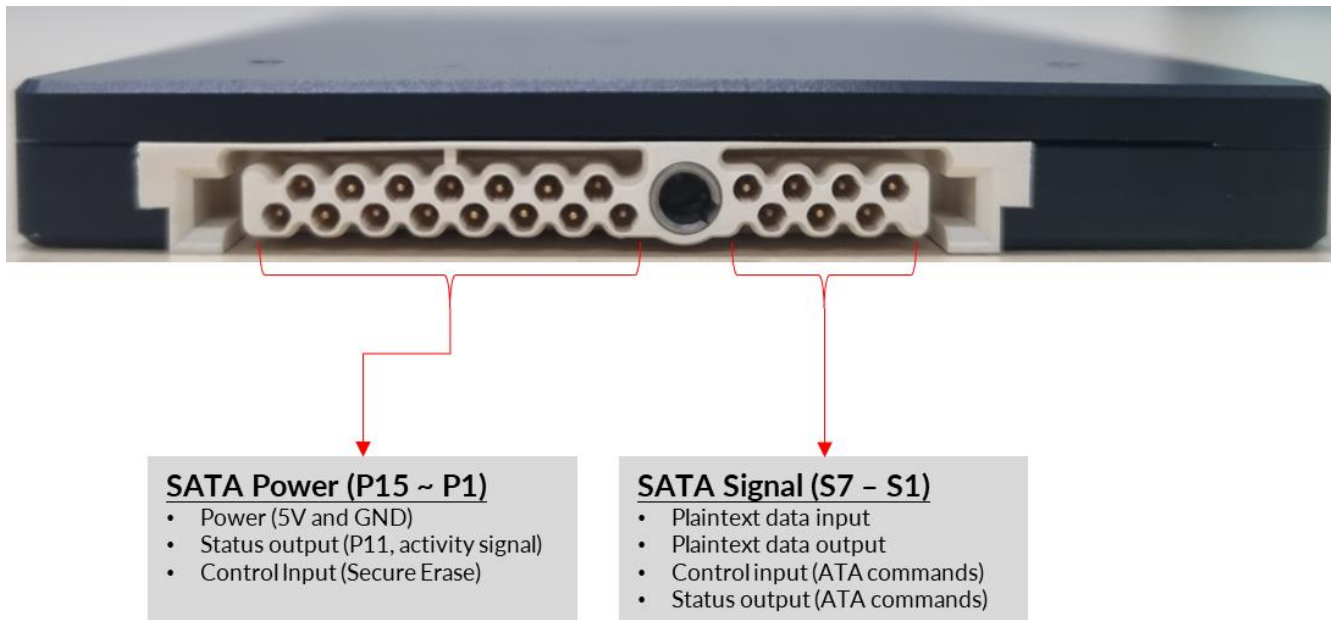
Figure 17. Ports description of 2.5" RSATA products (NS361P250GCC0-1S, NS361P500GCC0-1S, NS369P01T0VC0-1S, NS369P02T0VC0-1S)
