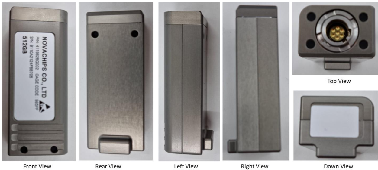
Figure 9. Removable Memory Module, Silver Color (NS361P125GCR4-1F-SL, NS369P250GVR4-1F-SL, NS369P500GVR4-1F-SL)
