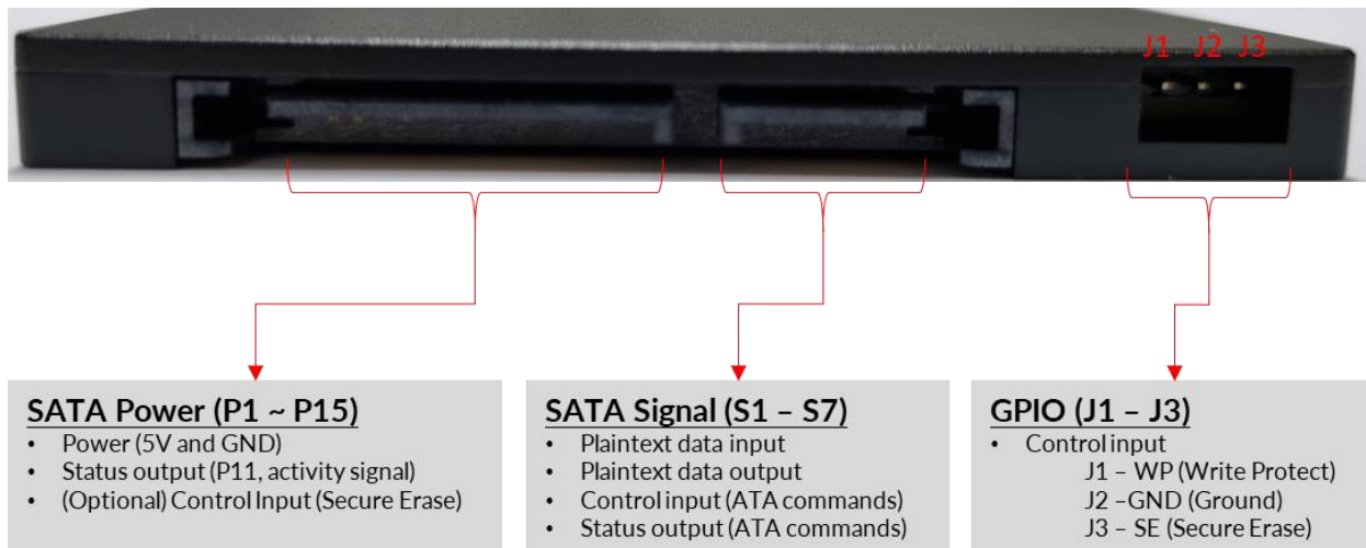
Figure 16. Ports description of 2.5” SATA products (NS361P500GCCR-1F, NS371P01TOCC1-1F, NS371P02TOCC1-1F, NS371P04TOCC1-1F, NS371P08TOCC0-1F, NS371P10TOCC0-1F, NS379P16TOVCO-1F, and NS379P20TOVCO-1F)
