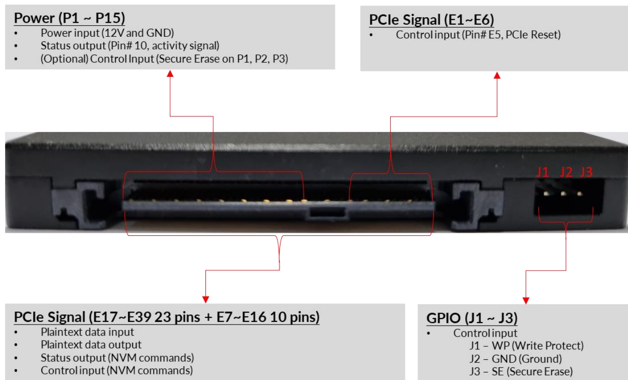
Figure 22. Ports description of PCIe U.2 SSD module (NS571P01TOCC0-1F, NS571P02TOCC0-1F, NS571P04TOCC0-1F, NS571P08TOCC0-1F)
