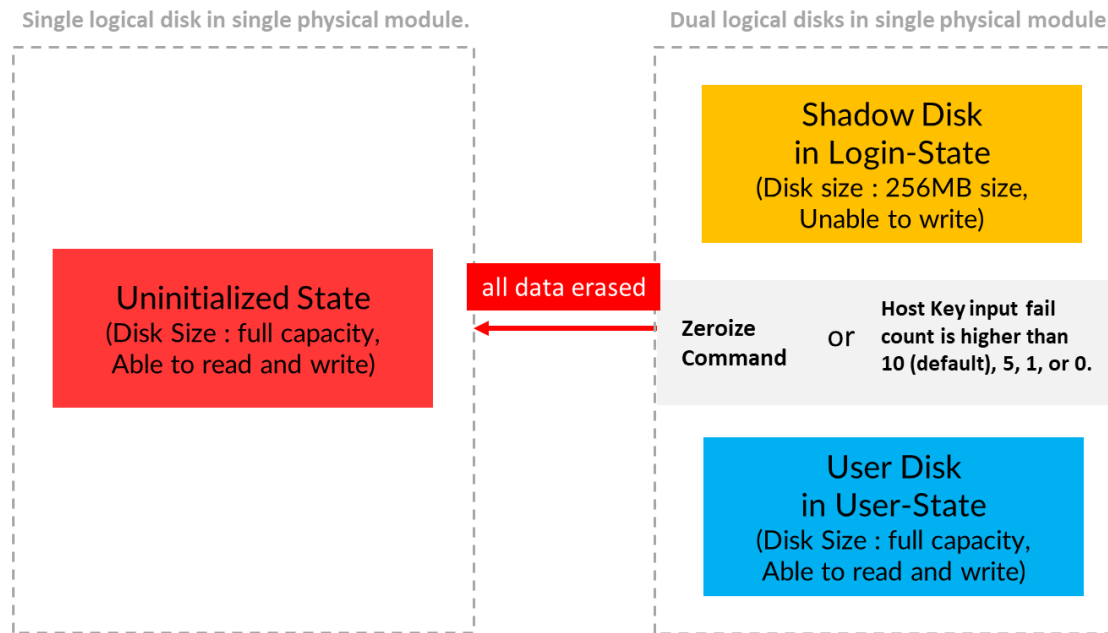
Figure 24. Simplified Diagram of TOE operation at zeroization
