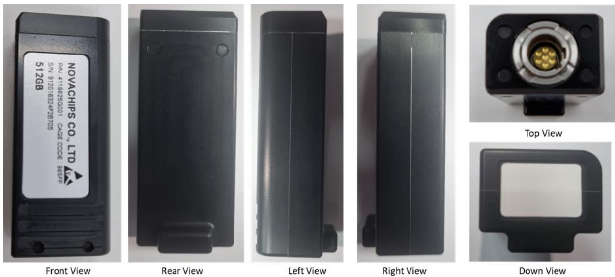
Figure 8. Removable Memory Module, Black Color (NS361P125GCR4-1F, NS369P250GVR4-1F, NS369P500GVR4-1F)
