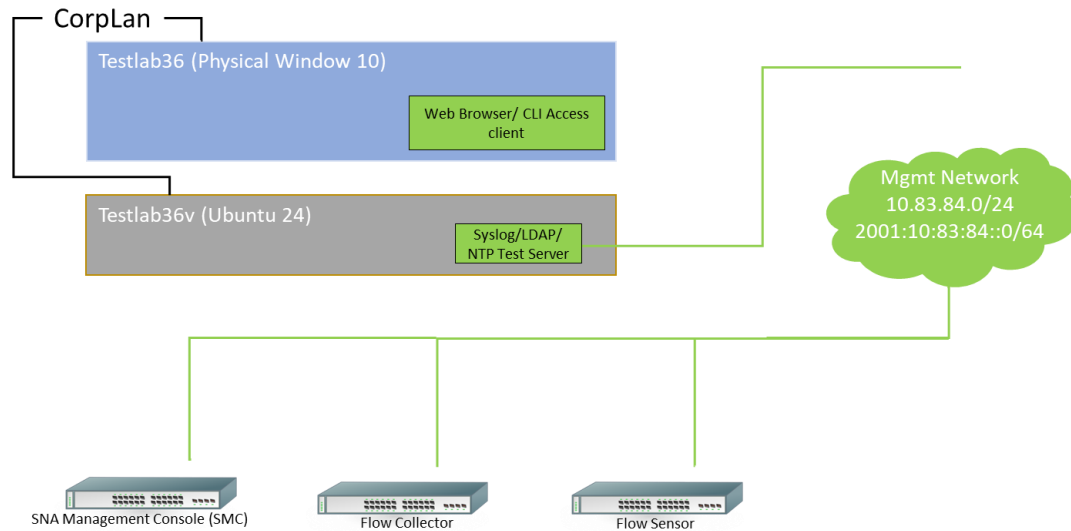
Figure 1 Physical Test Setup
